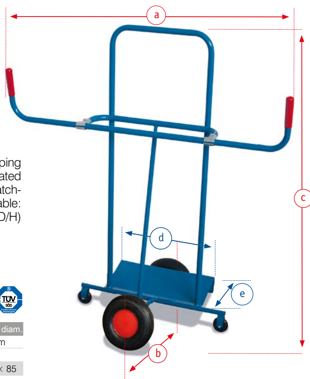
Sheet-material truck REF 138TA4001
