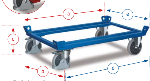
Dolly for pallets REF 138TA4003
