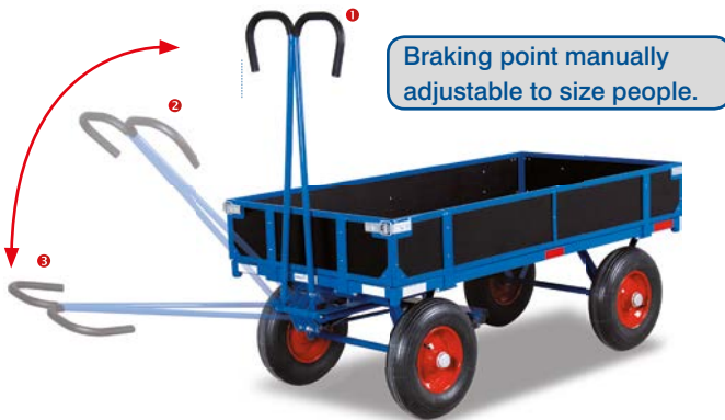
Hand platform trolley REF 138TA4102
