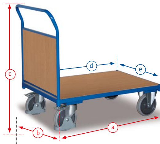
Single-end trolley REF 120TA9768
