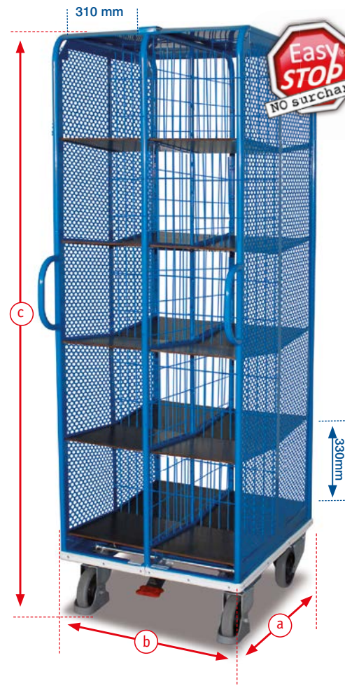
Document trolleys REF 161TA6805
